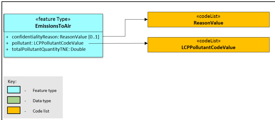
Figure 11- The EmissionsToAir feature type alongside connected data type and code lists
